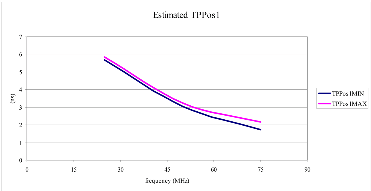
Figure 4. Estimated TPos1 over frequency
