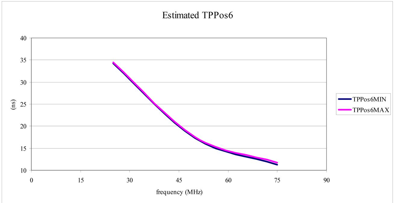
Figure 9. Estimated TPos6 over frequency
