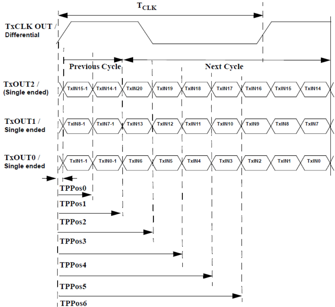
Figure 2. UT54LVDS217 TPPoS N Timing Diagram from Datasheet
