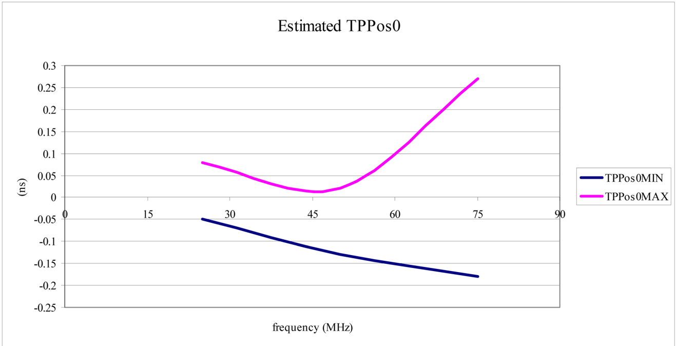
Figure 3. Estimated TPos0 over frequency
